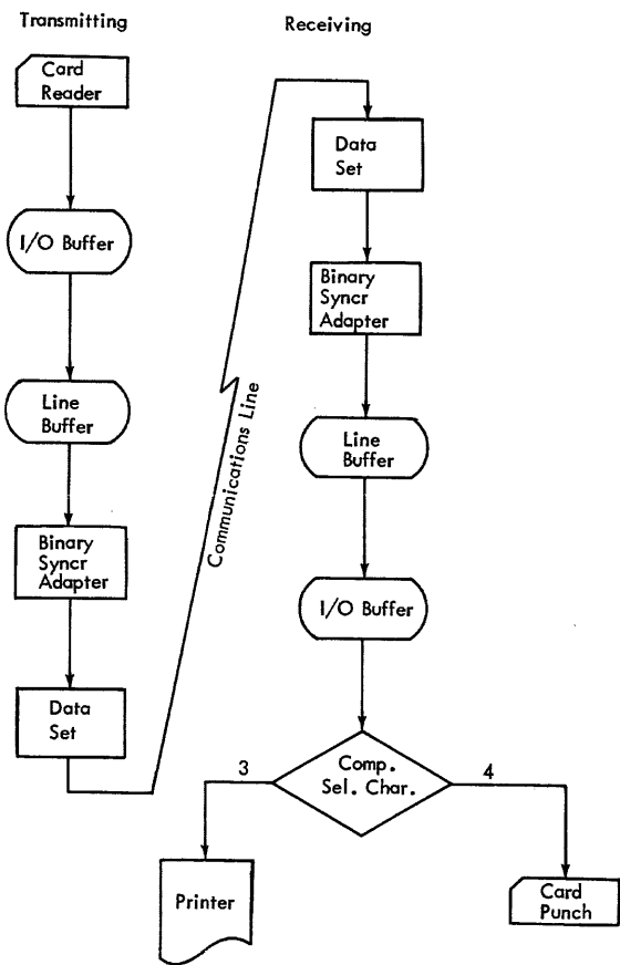
Figure 2. Data Flow, Terminal-to-Terminal Operation
