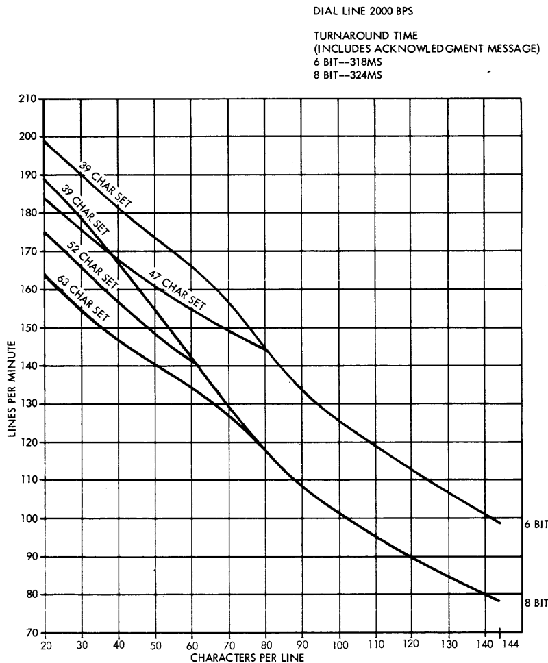
Figure 13. IBM 2780 Printer Approximate Throughput Rate -- Dial Line (See NOTE in Figure 7)
