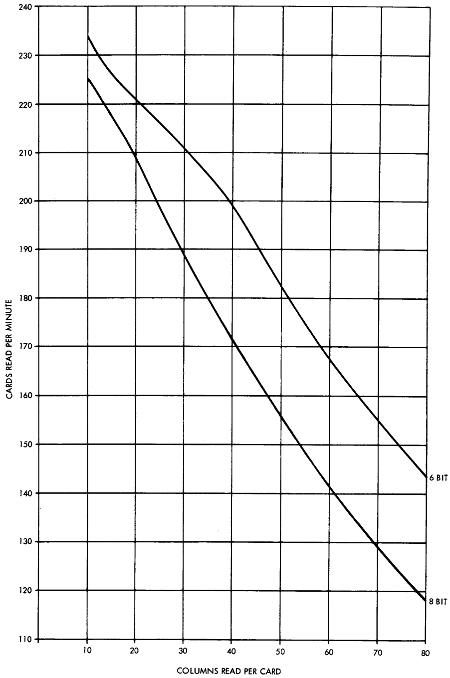
Figure 8. IBM 2780 Card Reader Approximate Throughput Rate--Dial Line (See NOTE in Figure 7)
