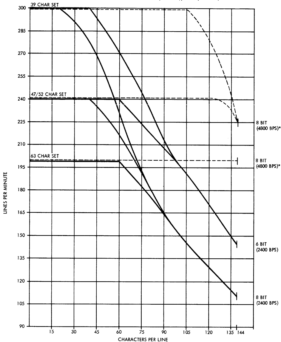
Figure 14. IBM 2780 Printer Approximate Throughput Rate -- Four-Wire Leased Line (See NOTE in Figure 7)
