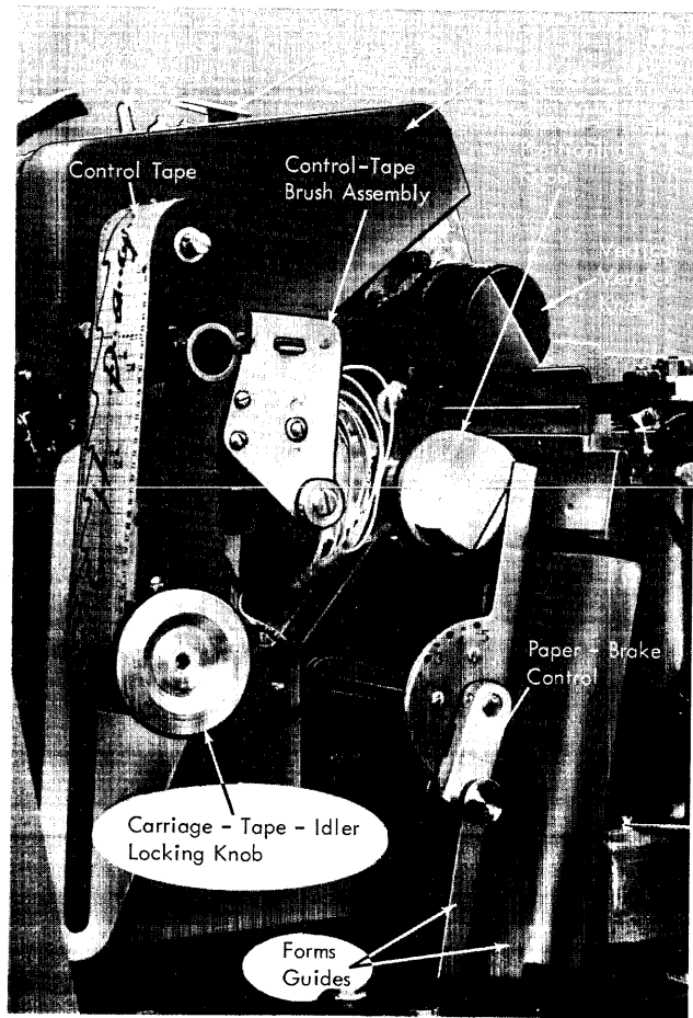
Figure 20. Printer Left-Hand Controls
