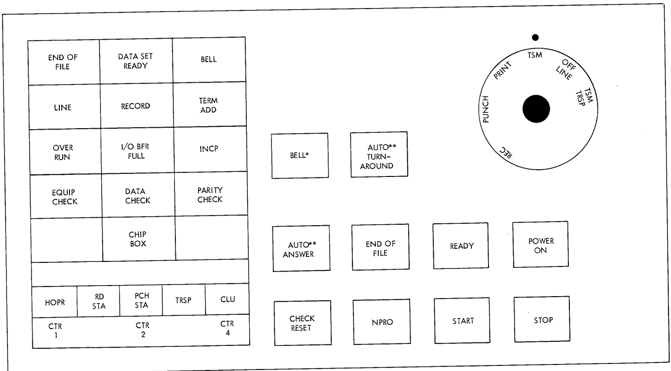
Figure 24. Card Read/Punch Operator Panel (Models 1, 2, and 4)
