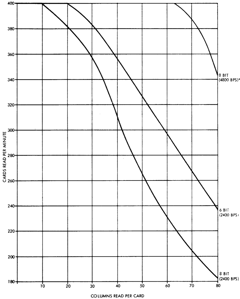
Figure 9. IBM 2780 Card Reader Approximate Throughput Rate--Four-Wire Leased Line (See NOTE in Figure 7)
