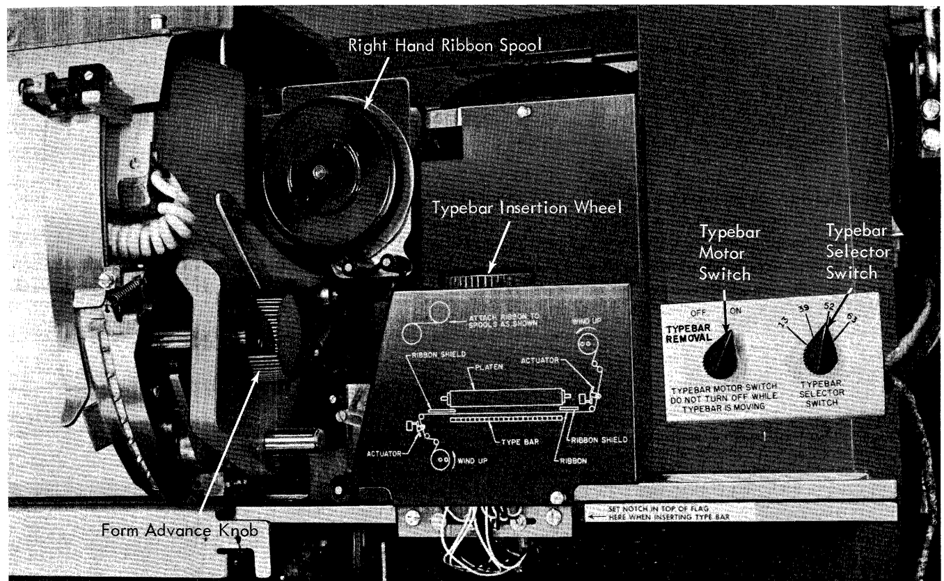
Figure 19. Printer Right-Hand Controls
