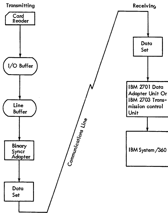
Figure 3. Data Flow, Terminal-to-Computer Operation
