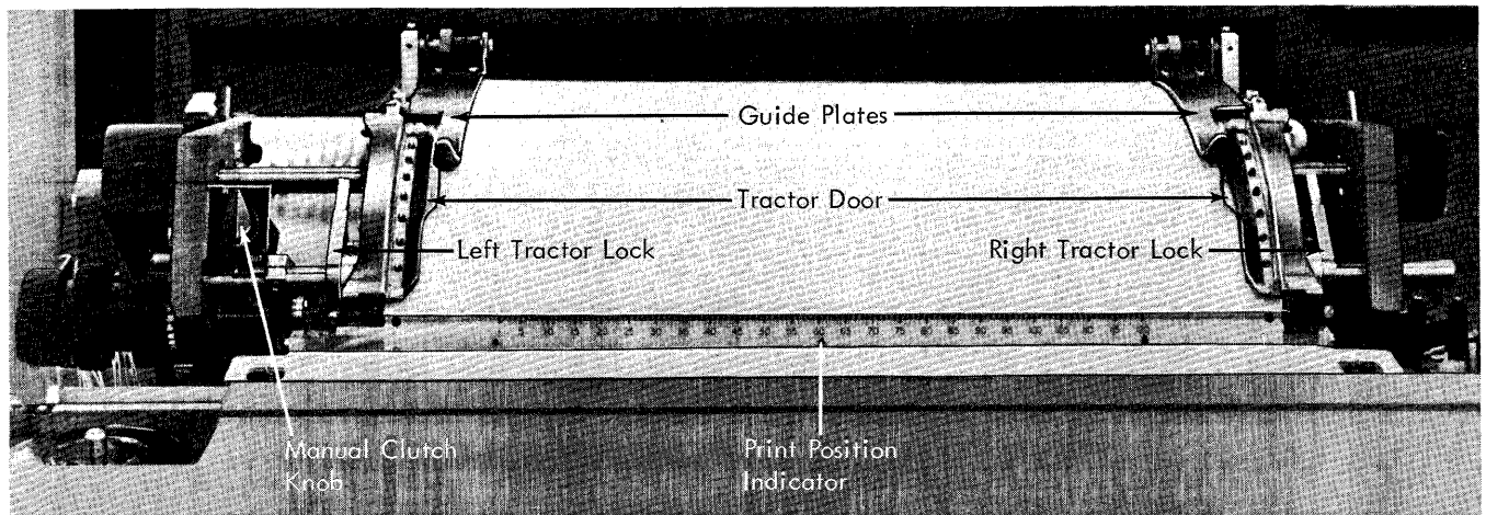
Figure 18. Tractor Feed
