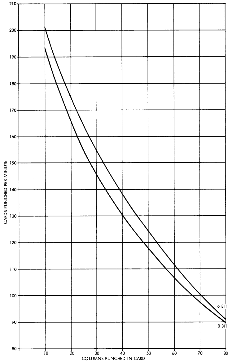
Figure 10. IBM 2780 Card Punch Approximate Throughput Rate--Dial Line (See NOTE in Figure 7)
