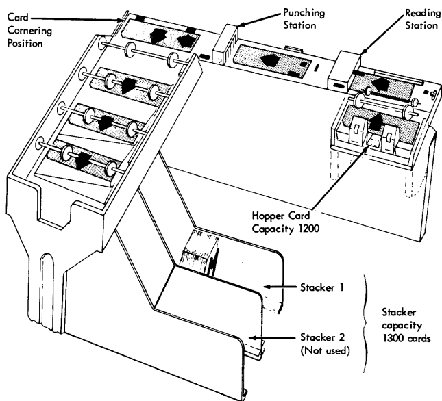
Figure 12. IBM 2780 Card Feed and Punch Schematic
