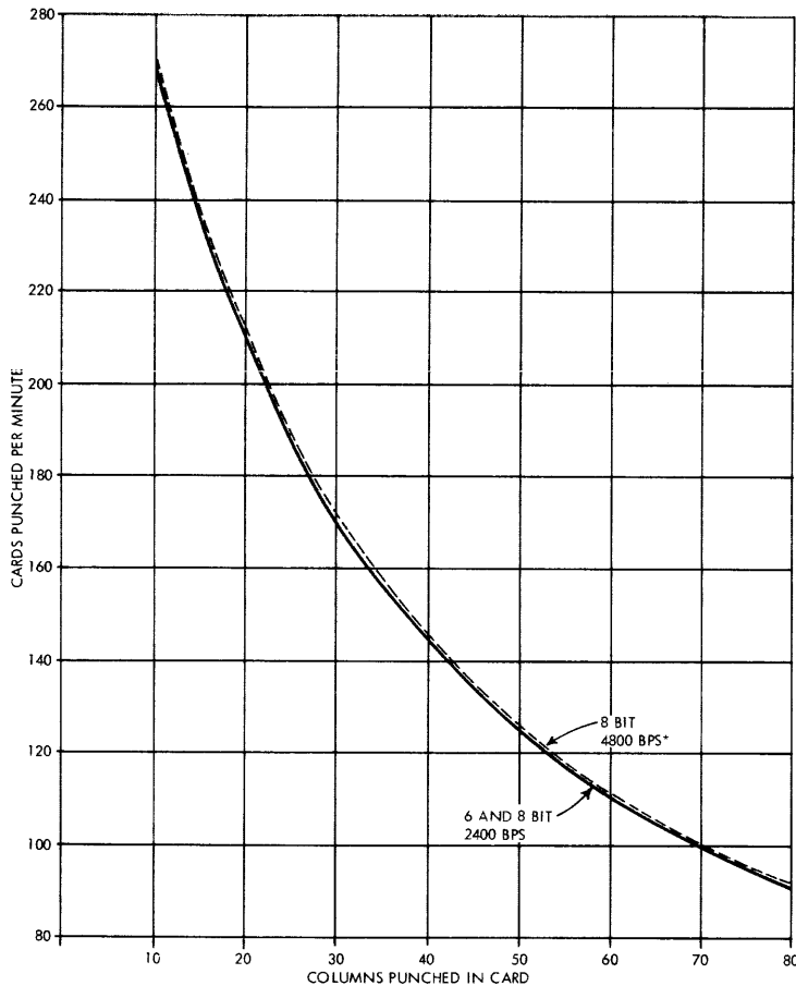
Figure 11. IBM 2780 Card Punch Approximate Throughput Rate -- Four-Wire Leased Line
